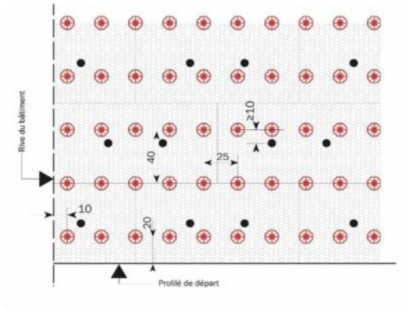
Figure 6c : Plan de chevillage 40 cm x 25 cm
