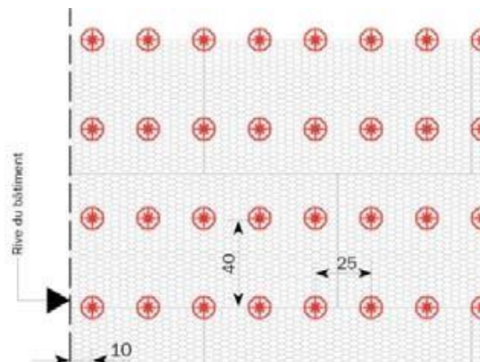
Figure 3c : Calepinage 40 cm x 25 cm
