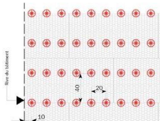
Figure 3d : Calepinage 40 cm x 20 cm
