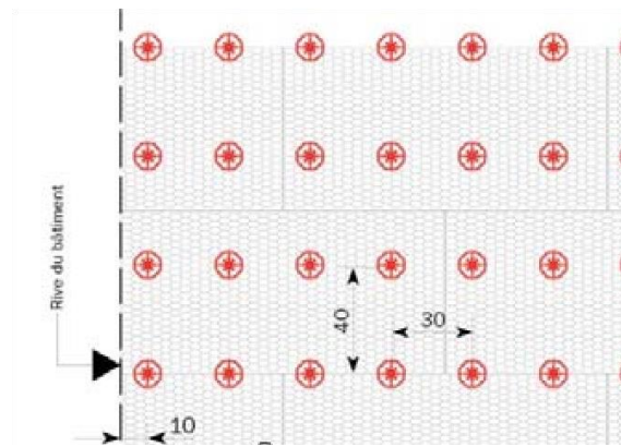
Figure 3b : Calepinage 40 cm x 30 cm
